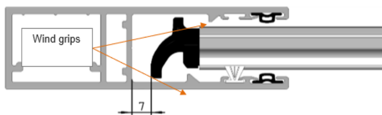
Fig. 5 – New GR105x35IE guider rail and SP/77WP side lock
