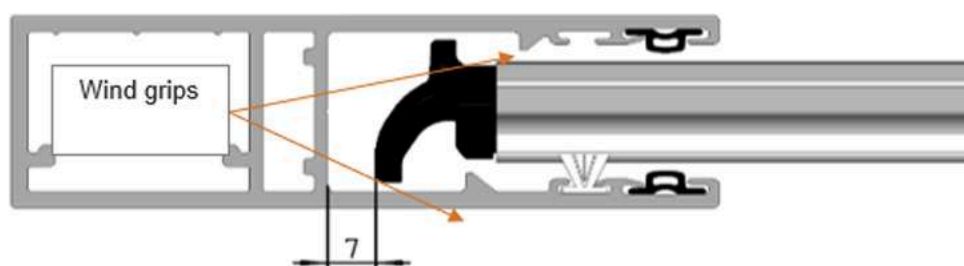
Fig. 5 – New GR105x35IE guider rail and SP/77WP side lock
