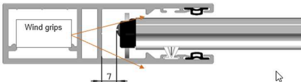
Fig. 6 – Previous version - GR100x35IE guide rail and SP/77-MSM (MSW) side lock
